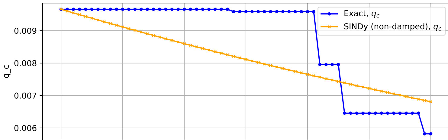
Trajectory No. 2702
