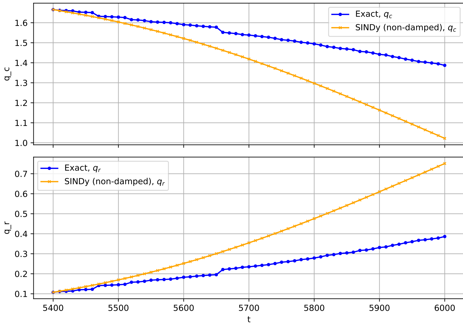
Trajectory No. 2712
