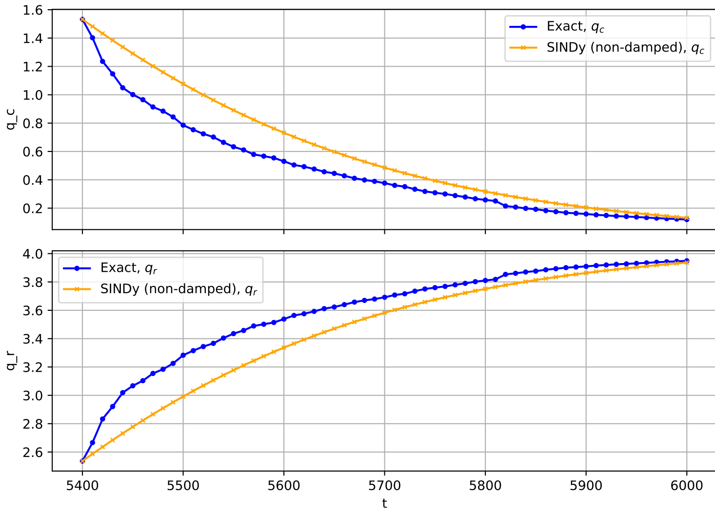
Trajectory No. 2753
