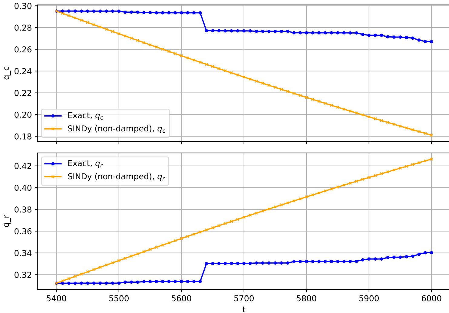
Trajectory No. 2794
