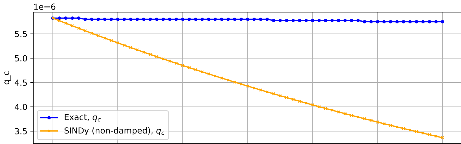
Trajectory No. 2821
