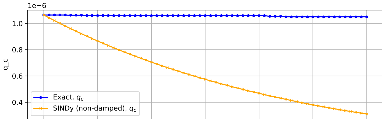
Trajectory No. 2828
