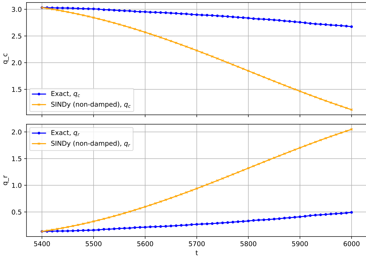
Trajectory No. 2870
