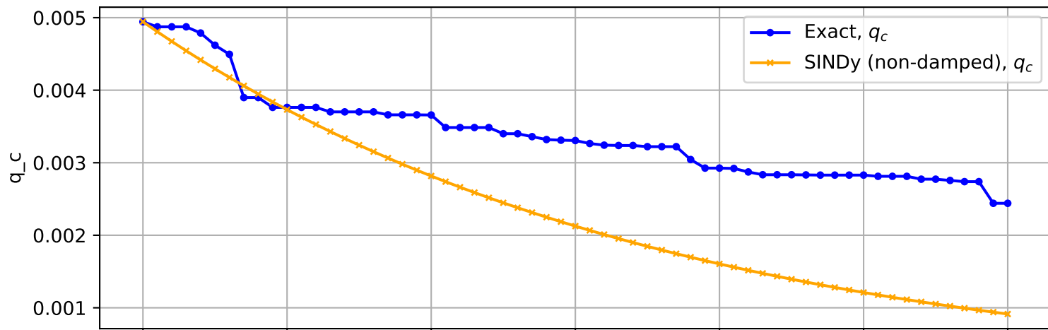
Trajectory No. 2951
