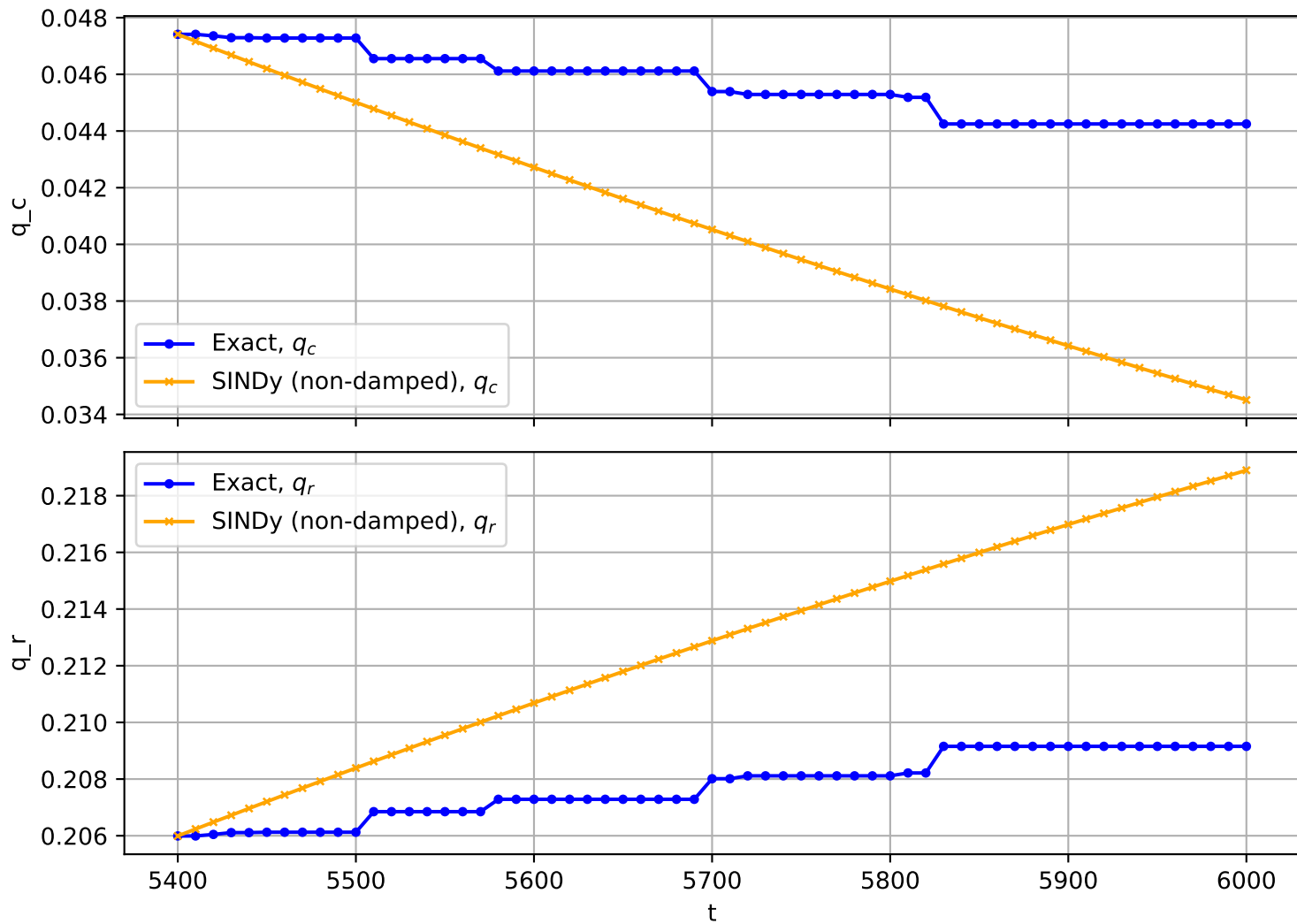
Trajectory No. 2954
