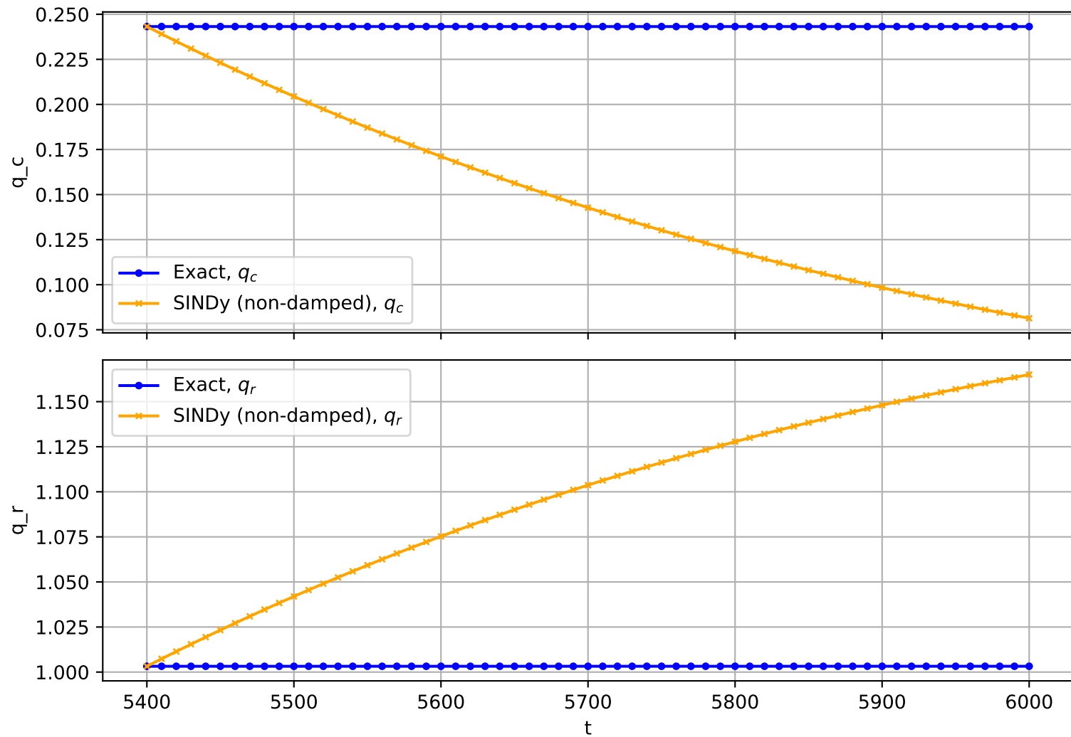
Trajectory No. 2963
