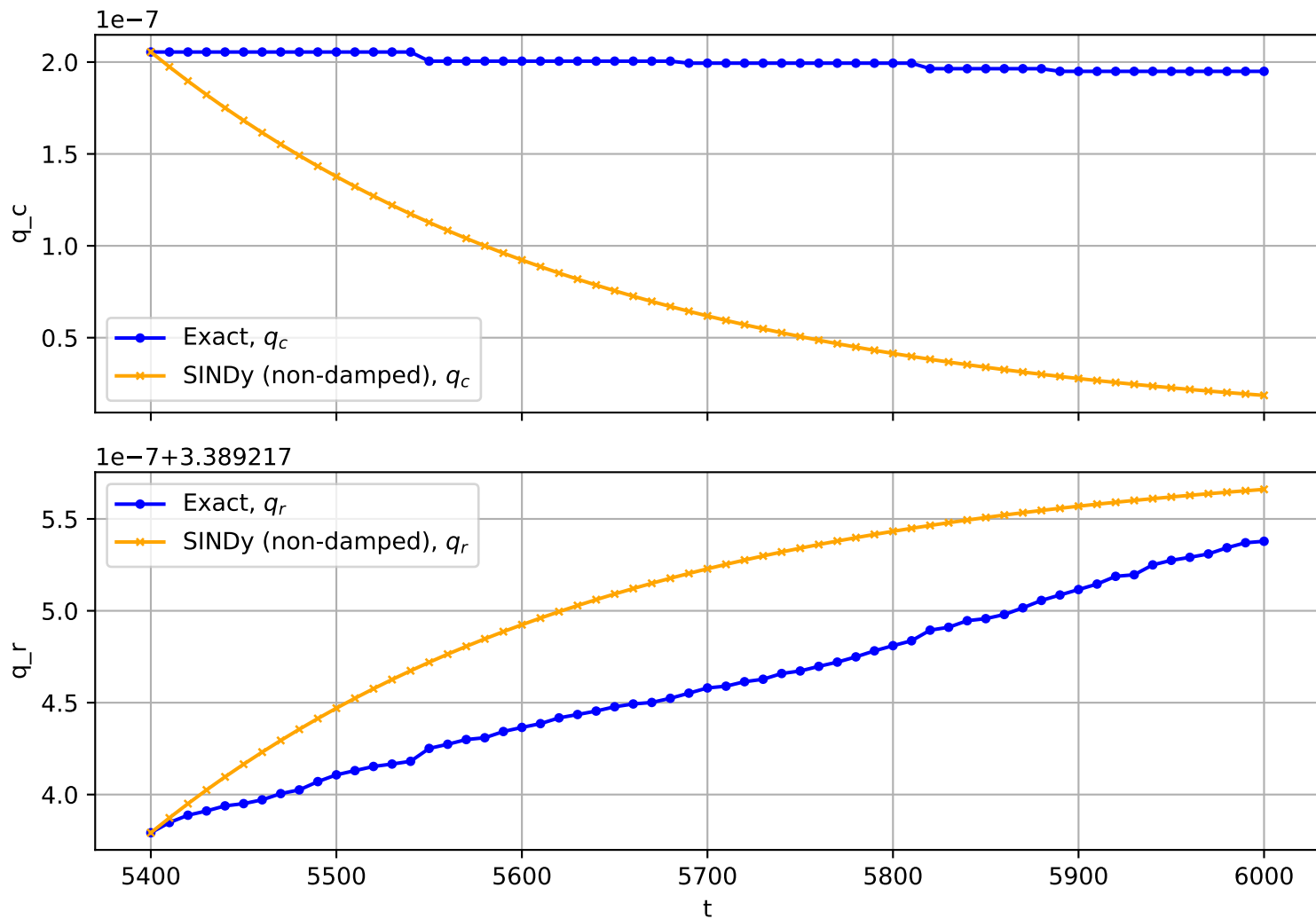
Trajectory No. 2969
