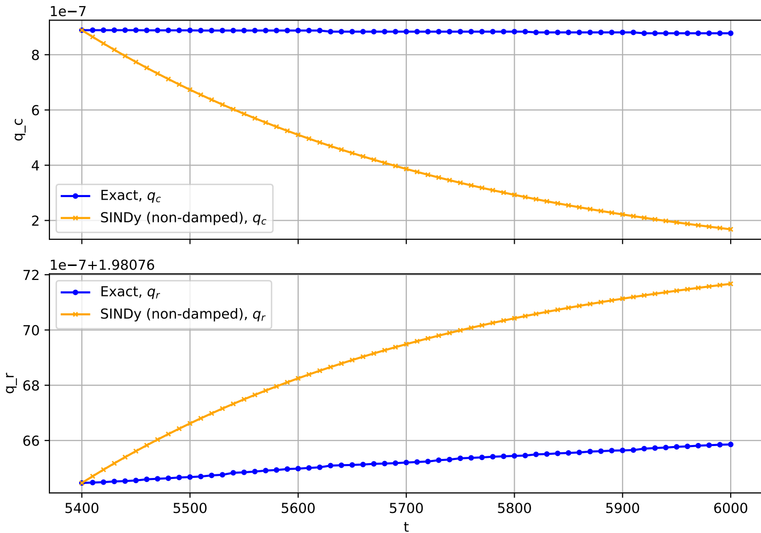
Trajectory No. 2970
