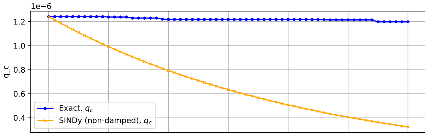
Trajectory No. 2981
