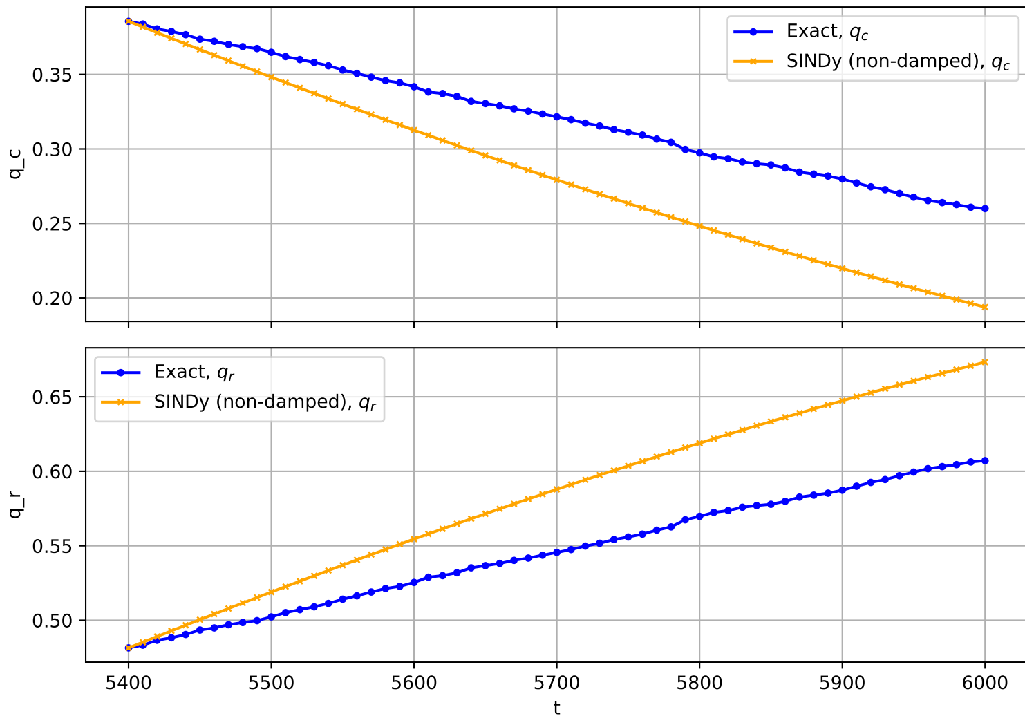
Trajectory No. 2984
