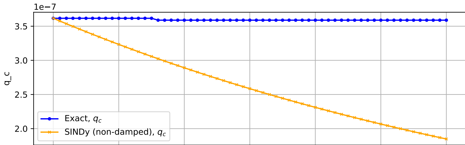
Trajectory No. 2989
