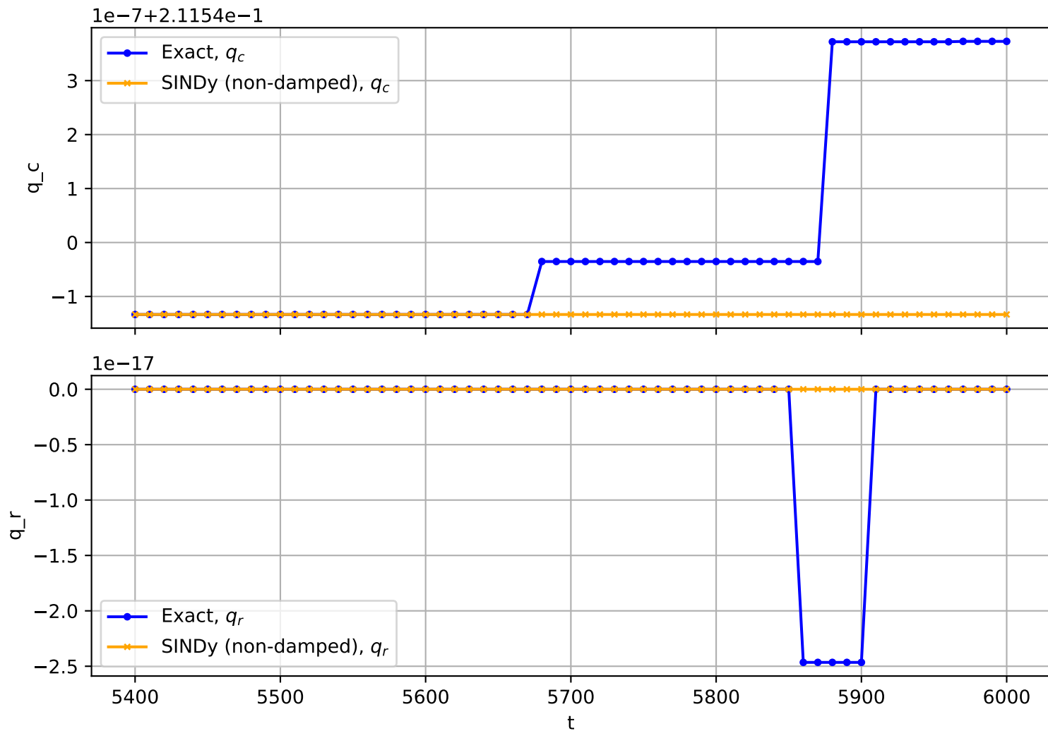
Trajectory No. 3071
