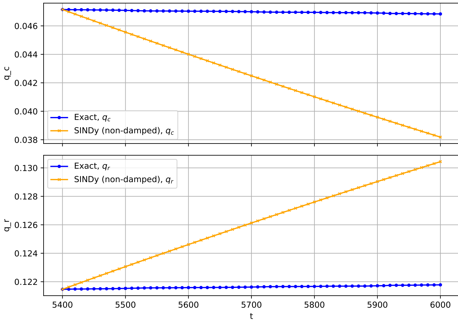
Trajectory No. 3078
