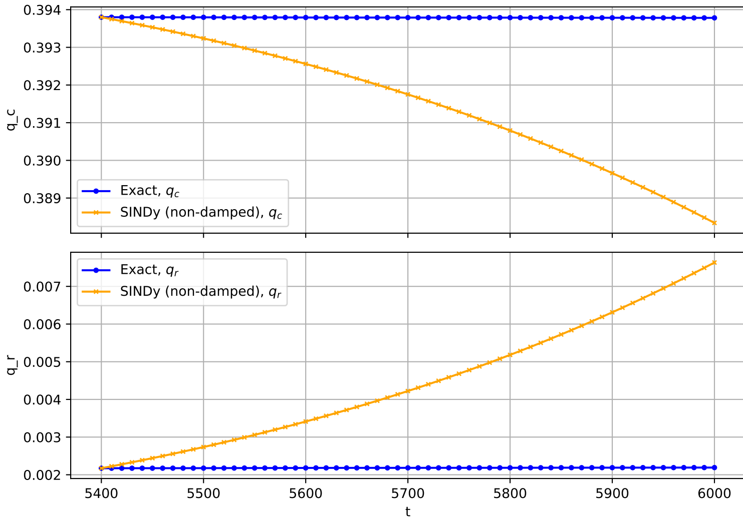
Trajectory No. 3163
