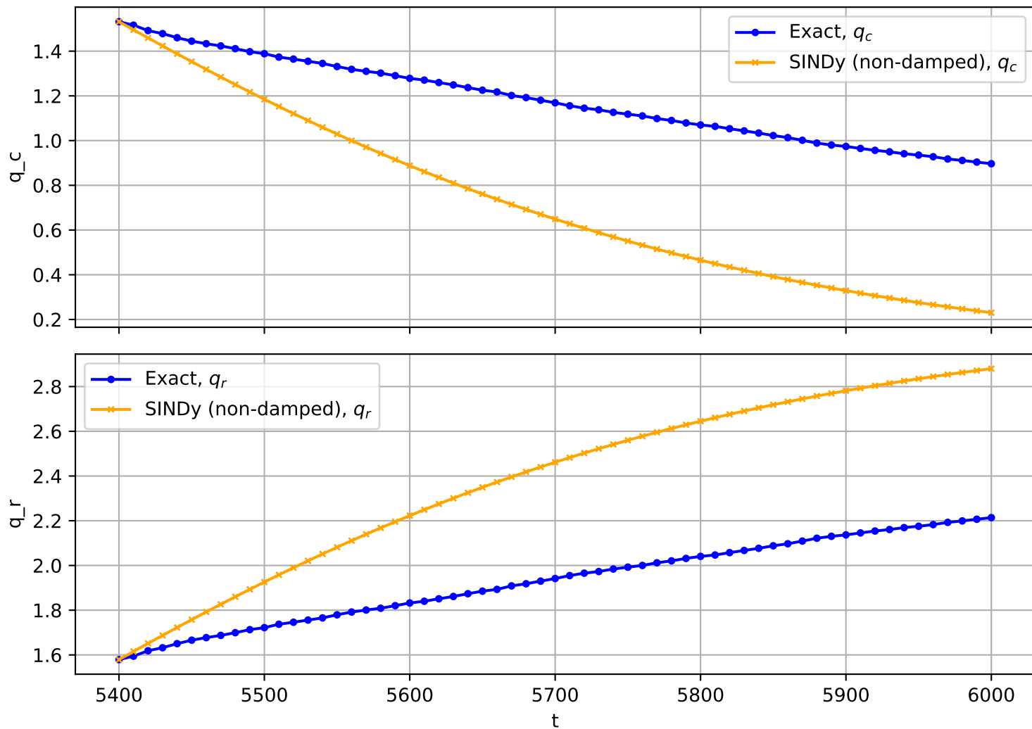
Trajectory No. 3196
