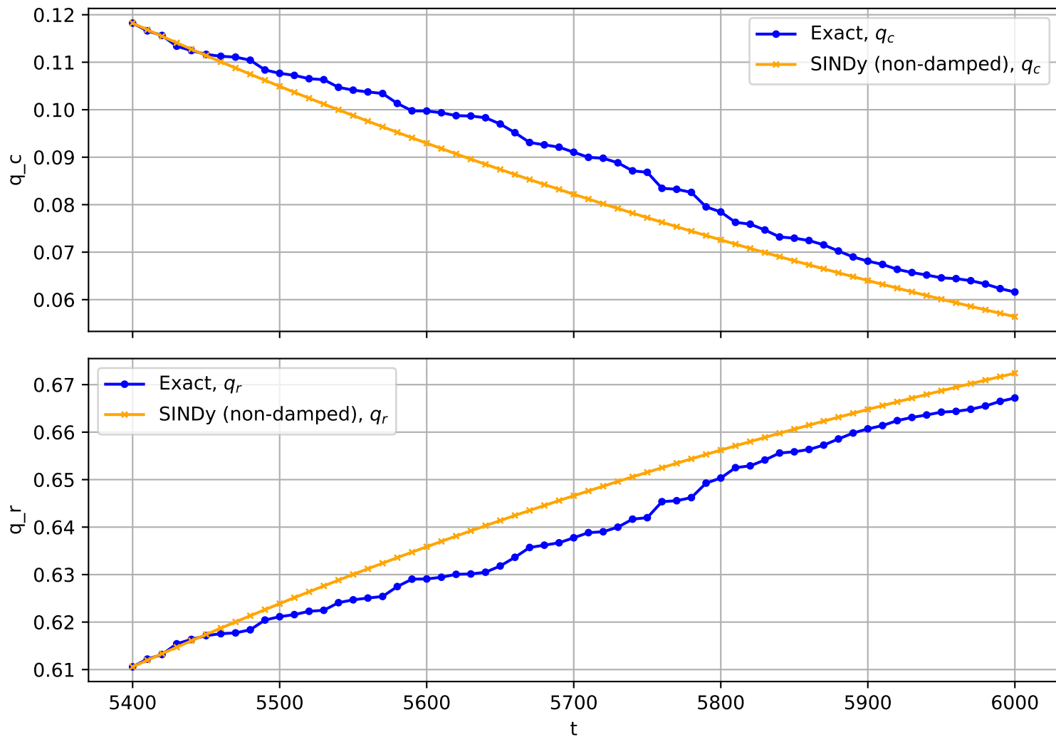
Trajectory No. 33
