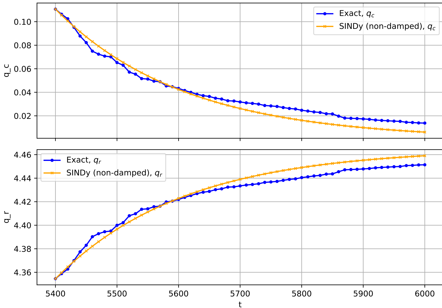
Trajectory No. 3366
