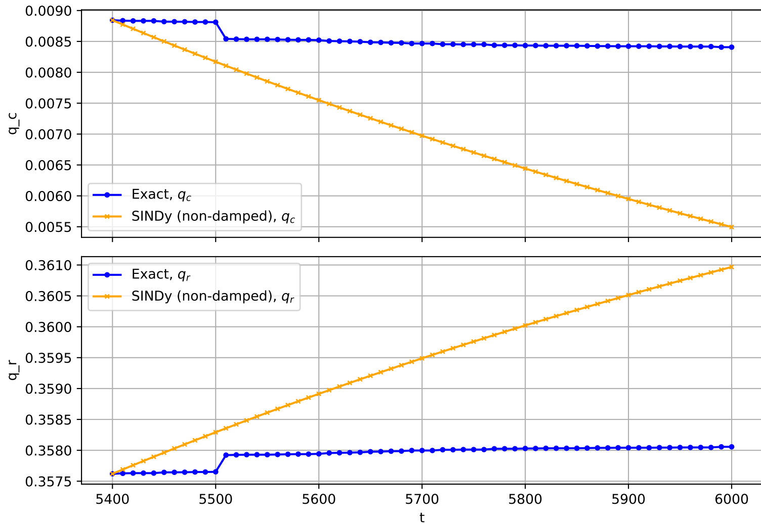
Trajectory No. 3431
