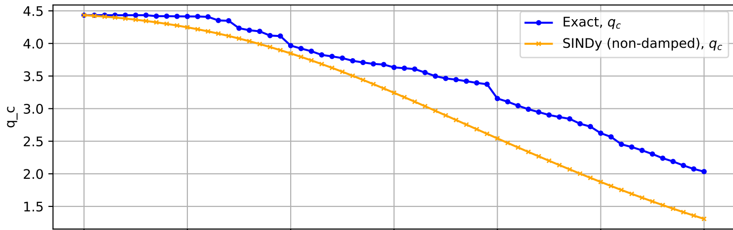
Trajectory No. 3458
