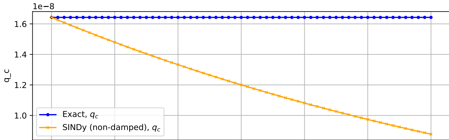
Trajectory No. 3492
