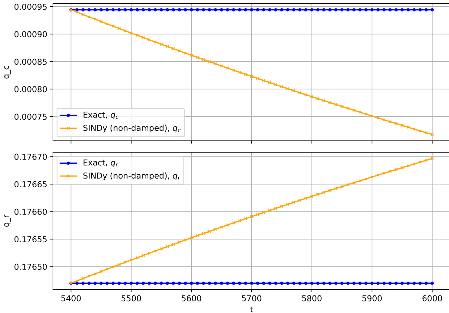
Trajectory No. 3502
