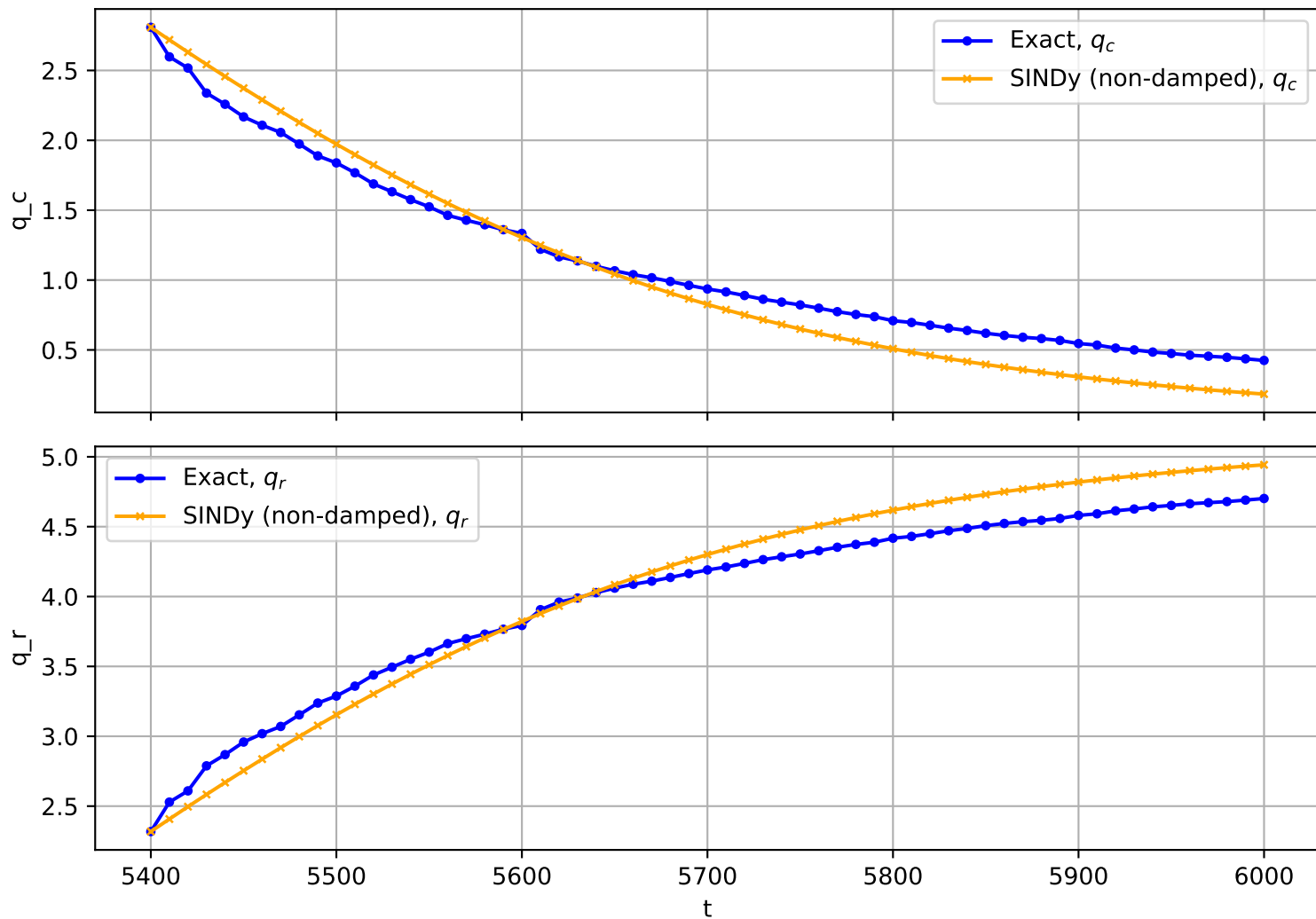
Trajectory No. 379
