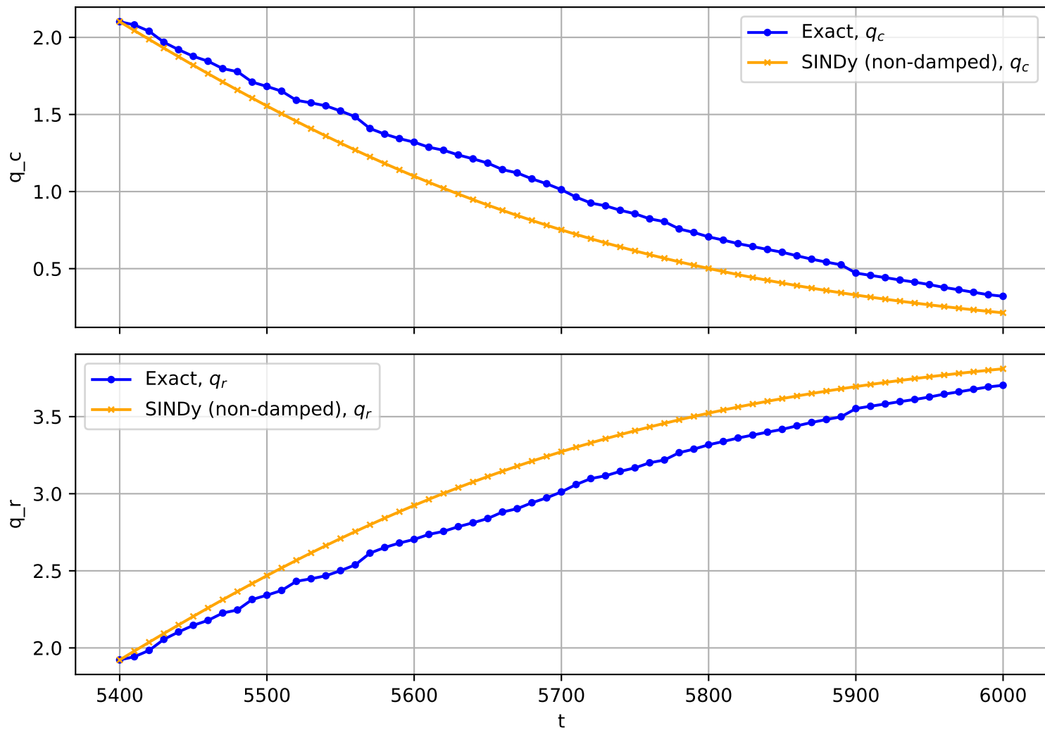
Trajectory No. 384
