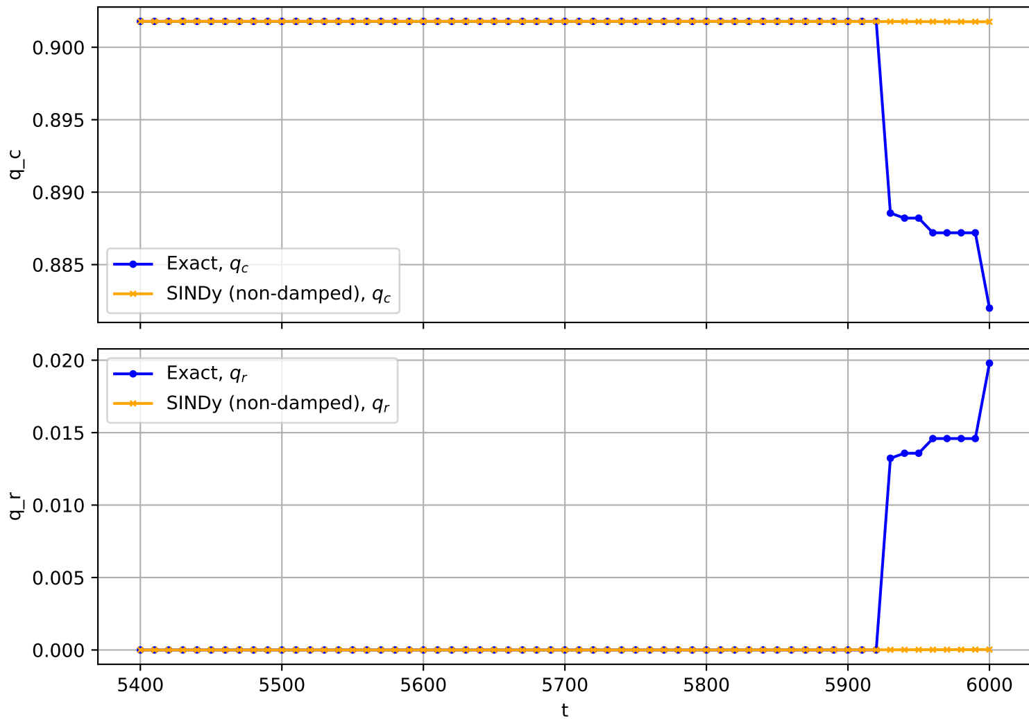
Trajectory No. 409
