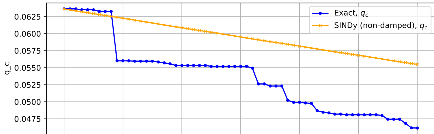
Trajectory No. 443
