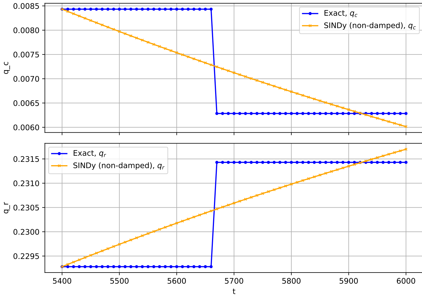
Trajectory No. 451
