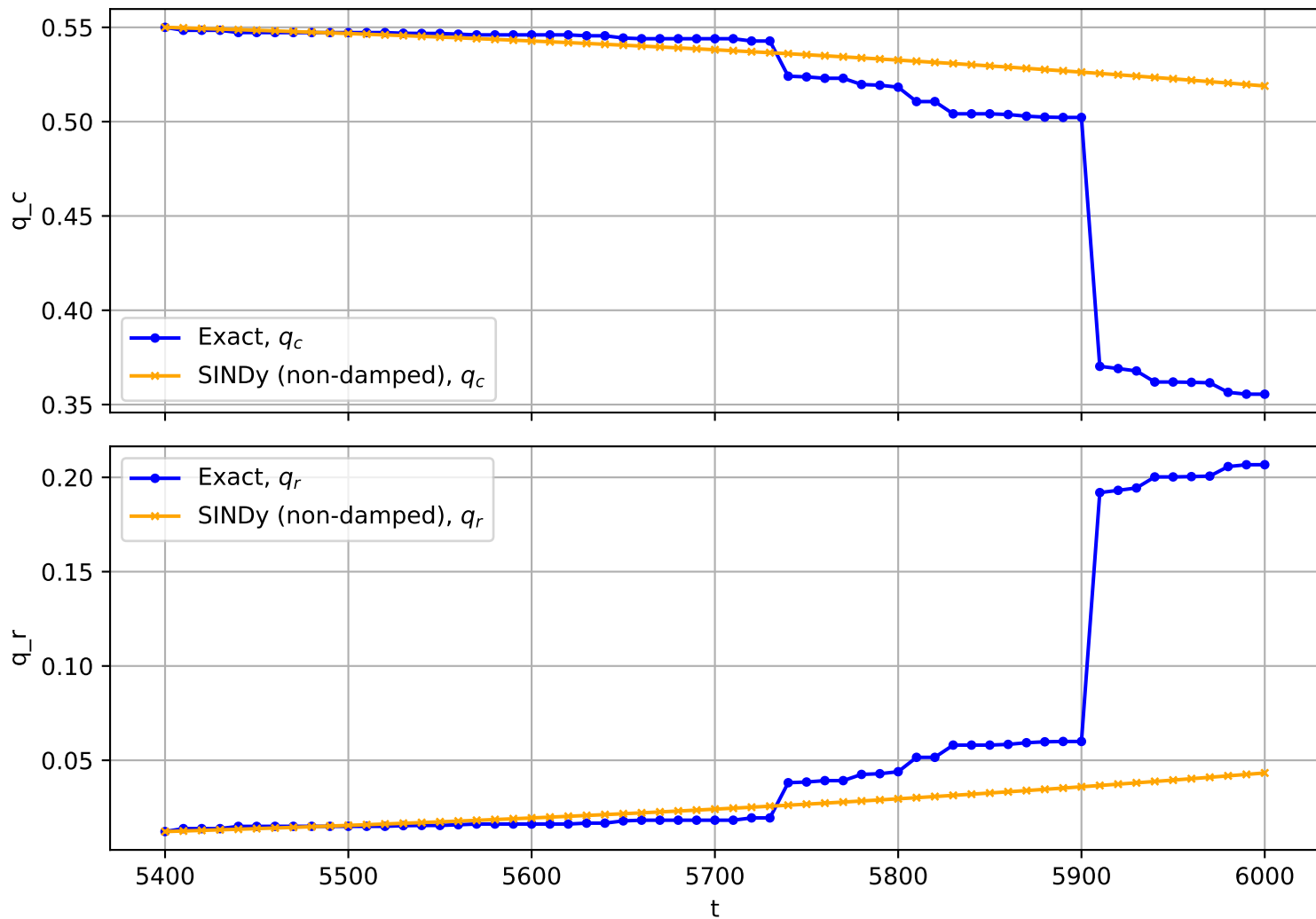
Trajectory No. 476
