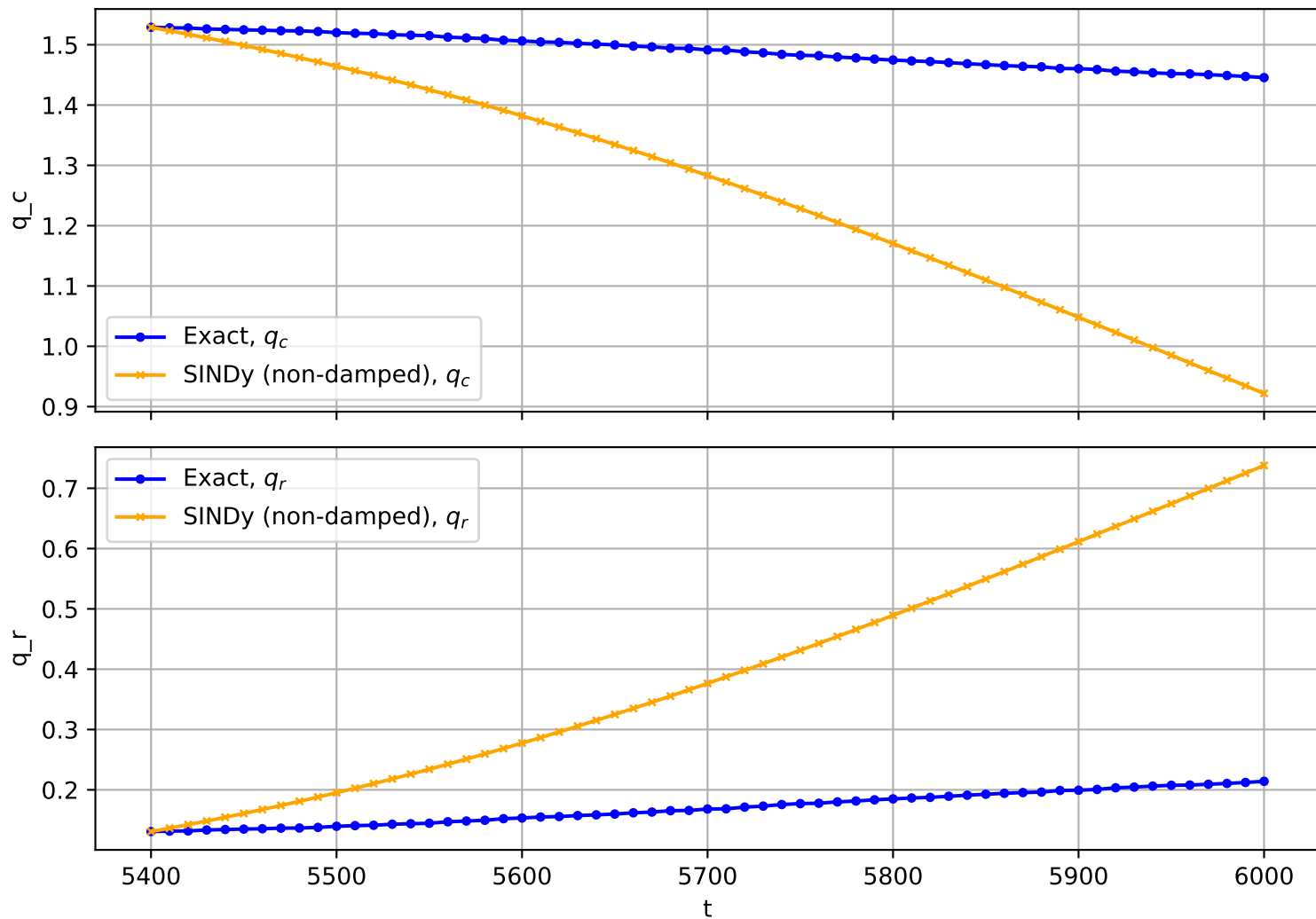
Trajectory No. 526
