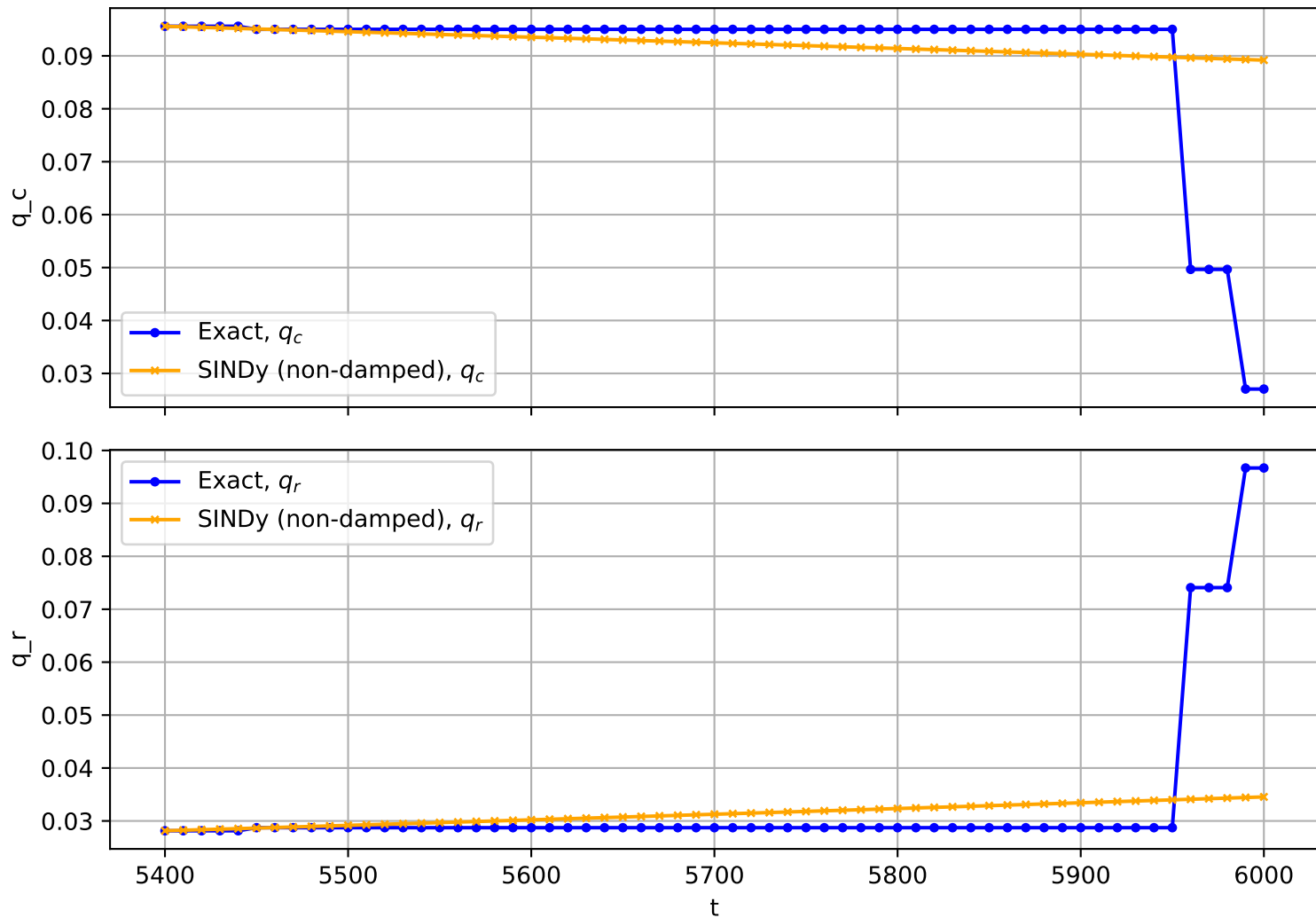
Trajectory No. 54
