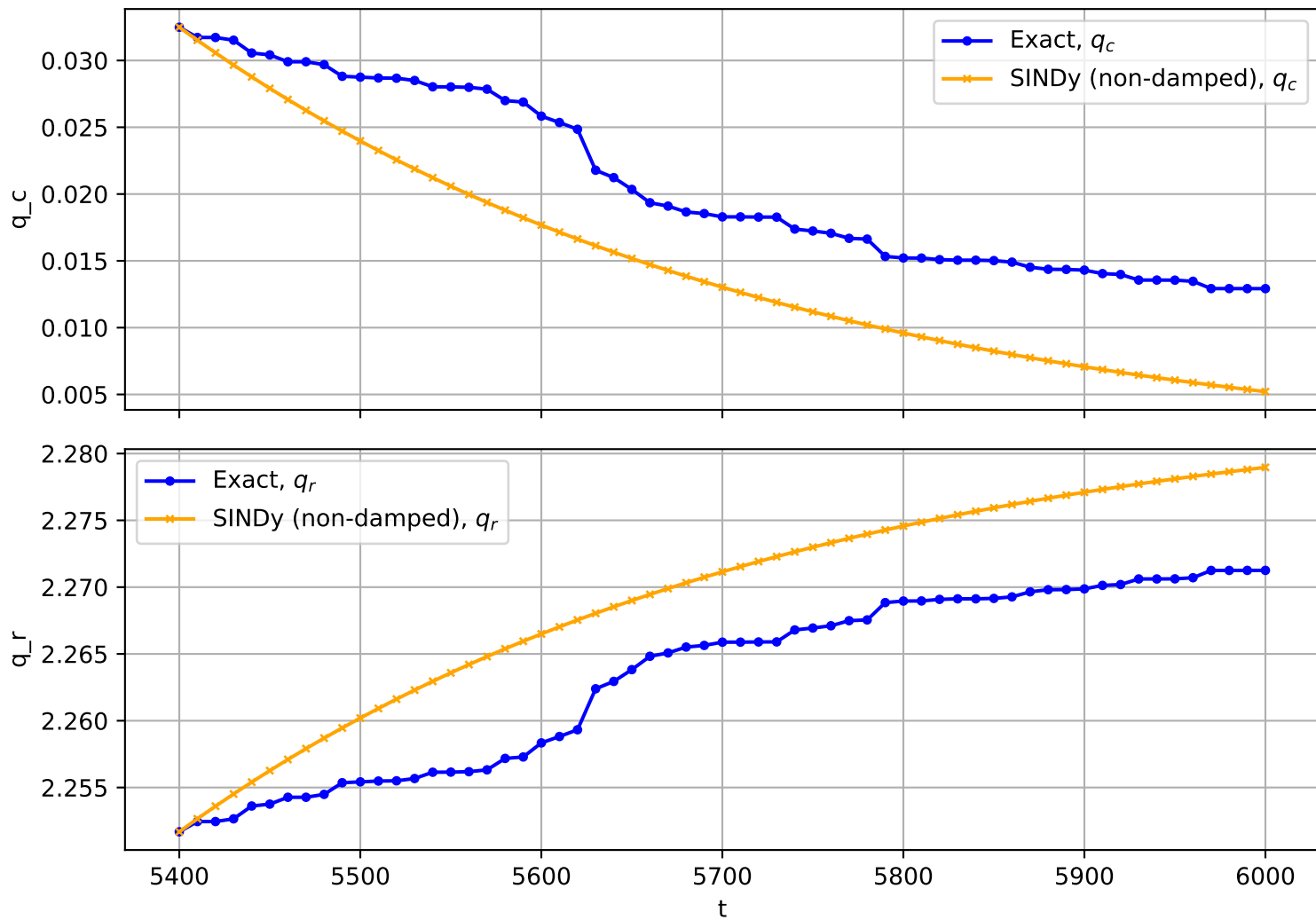
Trajectory No. 547
