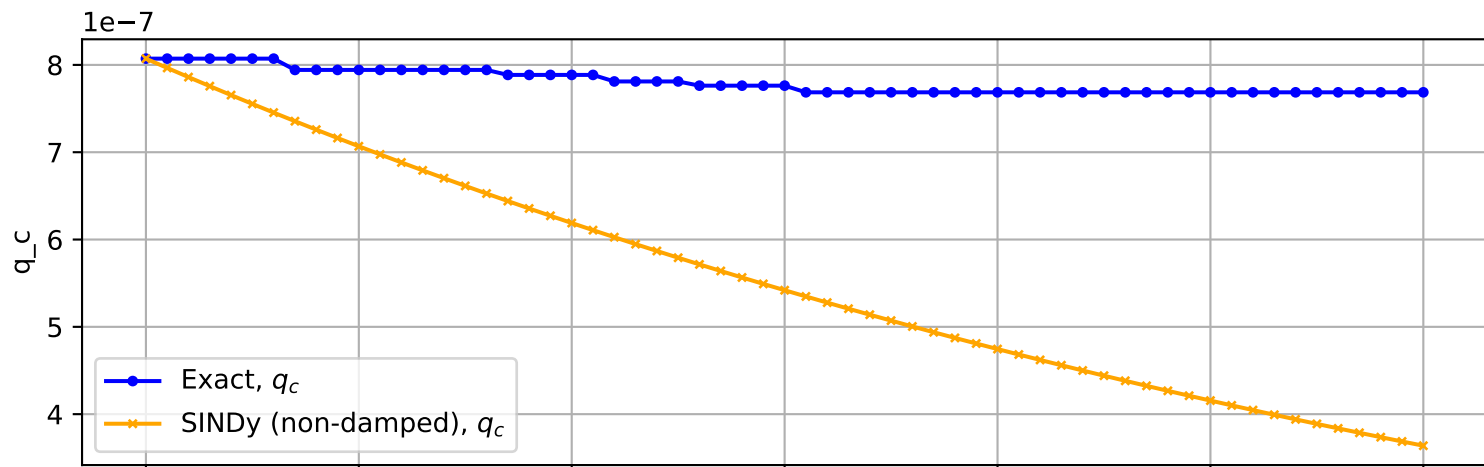
Trajectory No. 566
