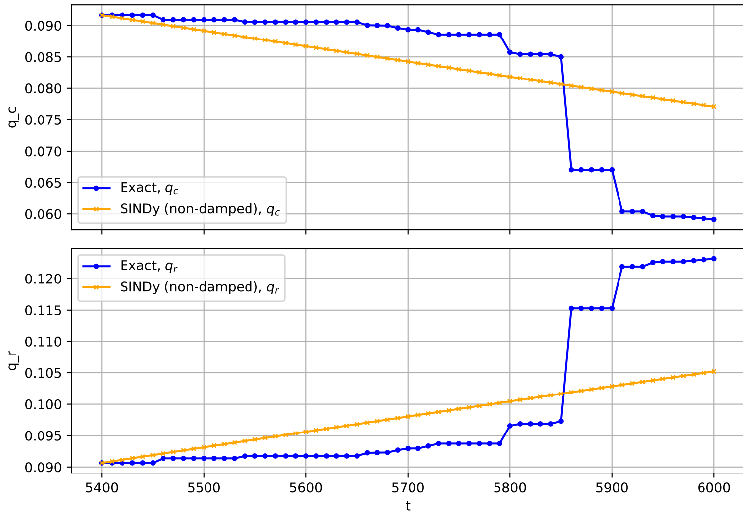
Trajectory No. 57
