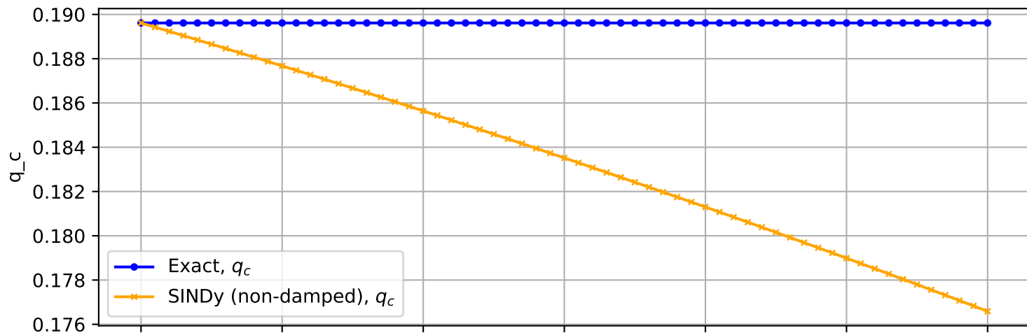
Trajectory No. 6
