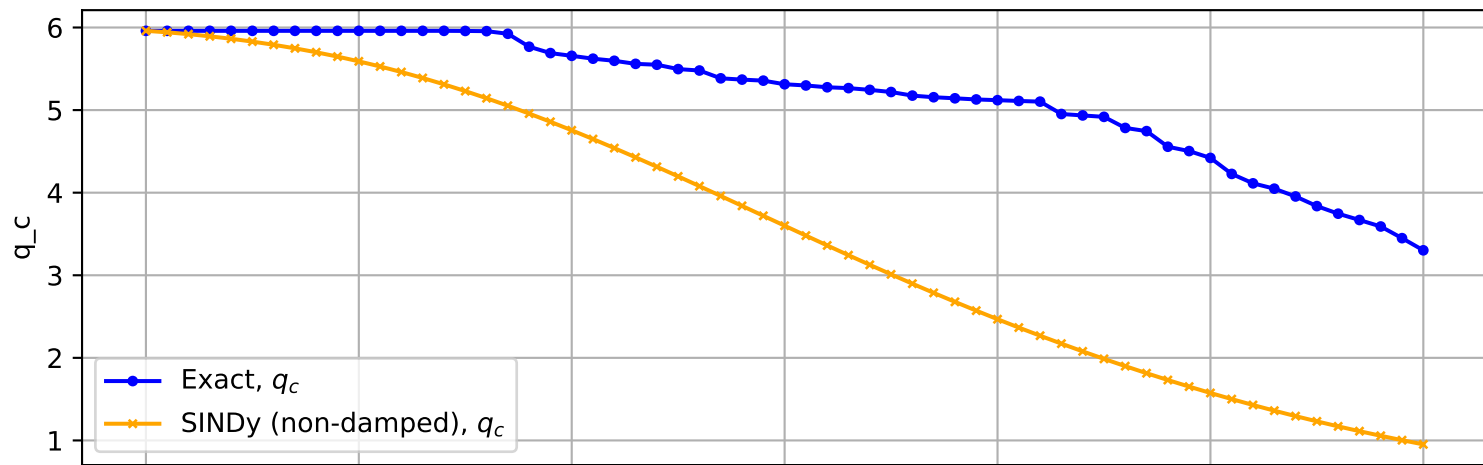
Trajectory No. 639
