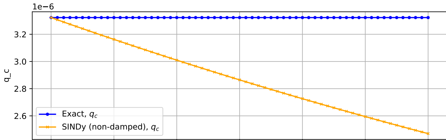
Trajectory No. 71
