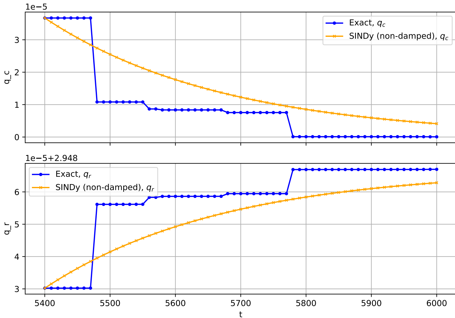
Trajectory No. 739
