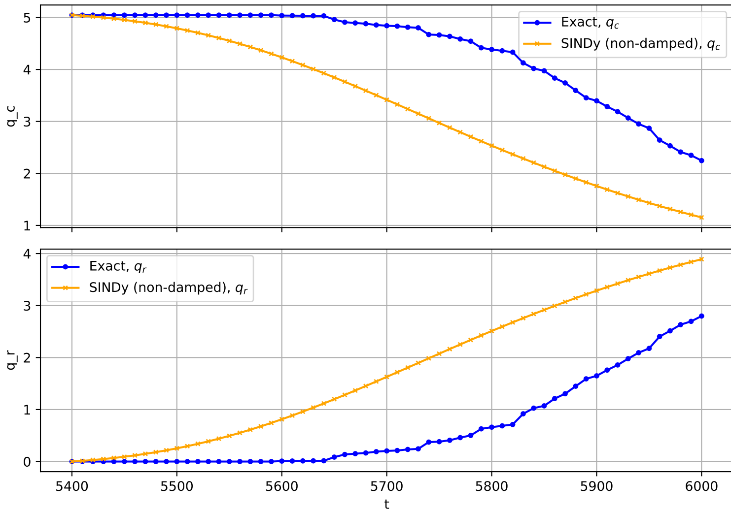
Trajectory No. 787
