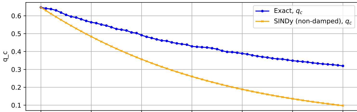
Trajectory No. 888
