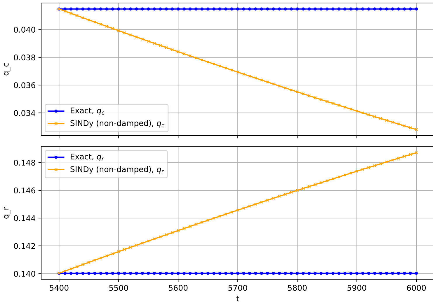
Trajectory No. 892
