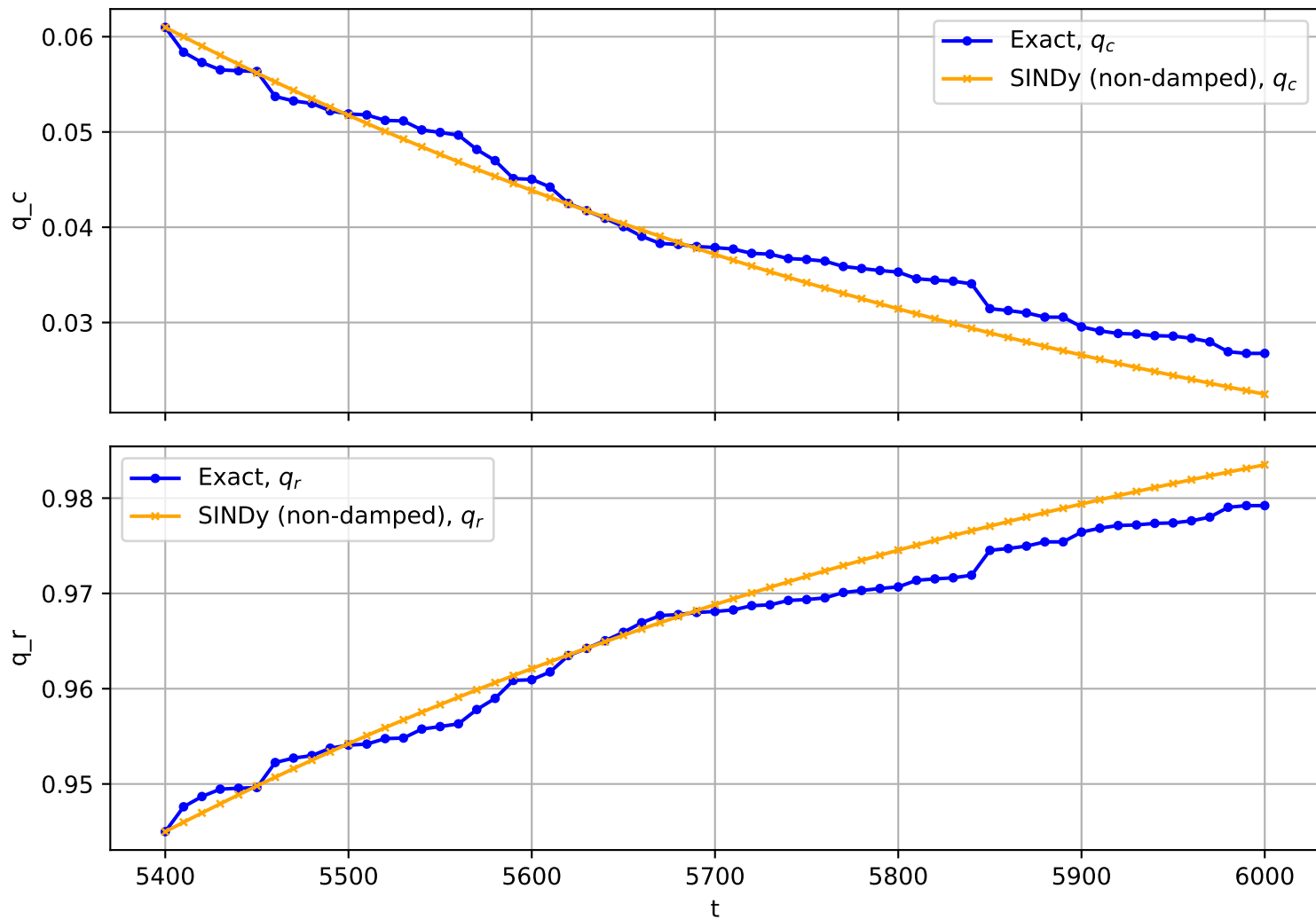
Trajectory No. 900
