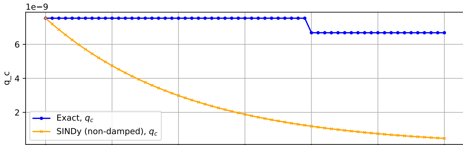
Trajectory No. 904
