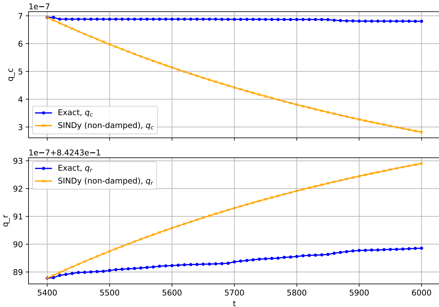
Trajectory No. 914
