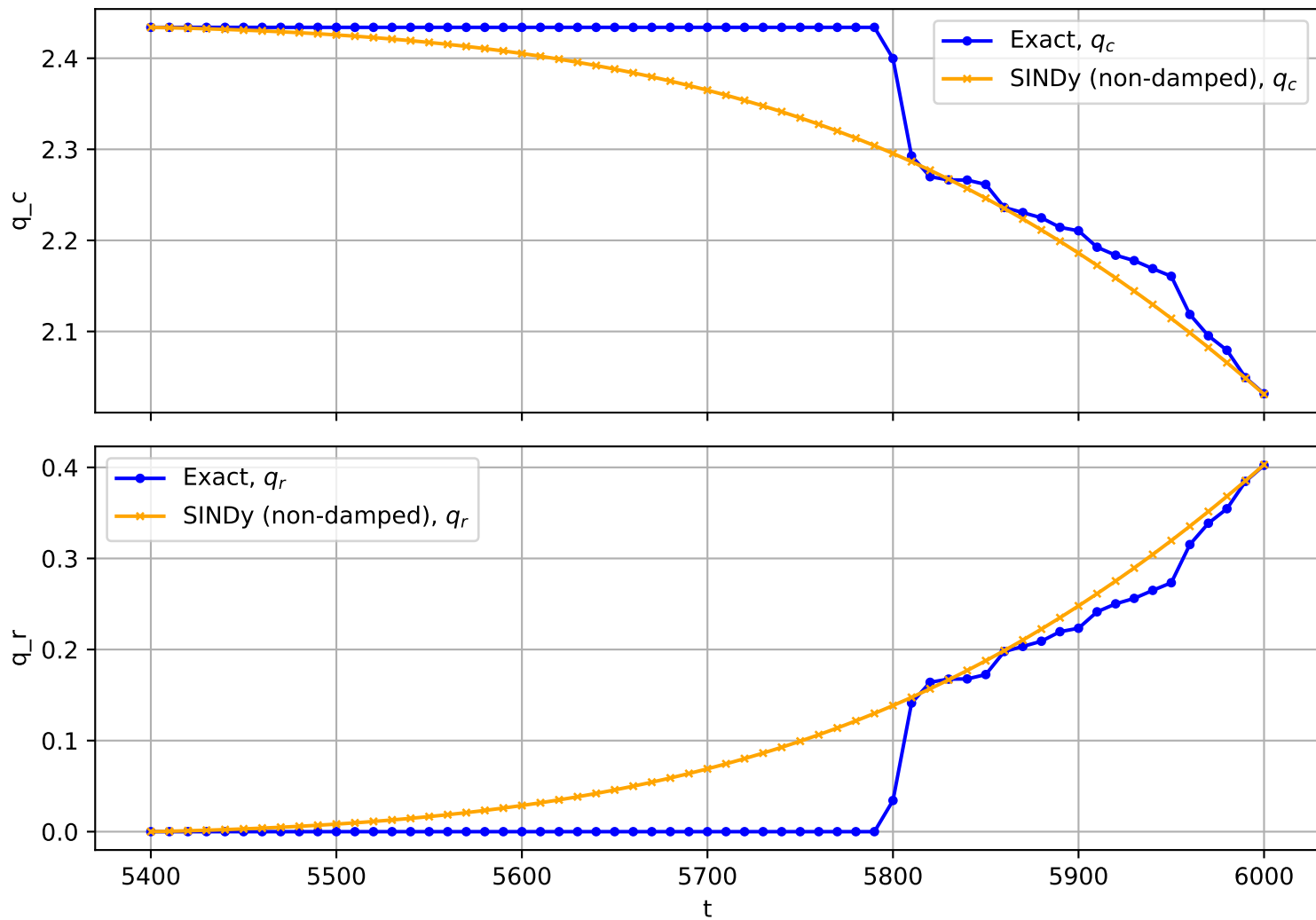
Trajectory No. 970
