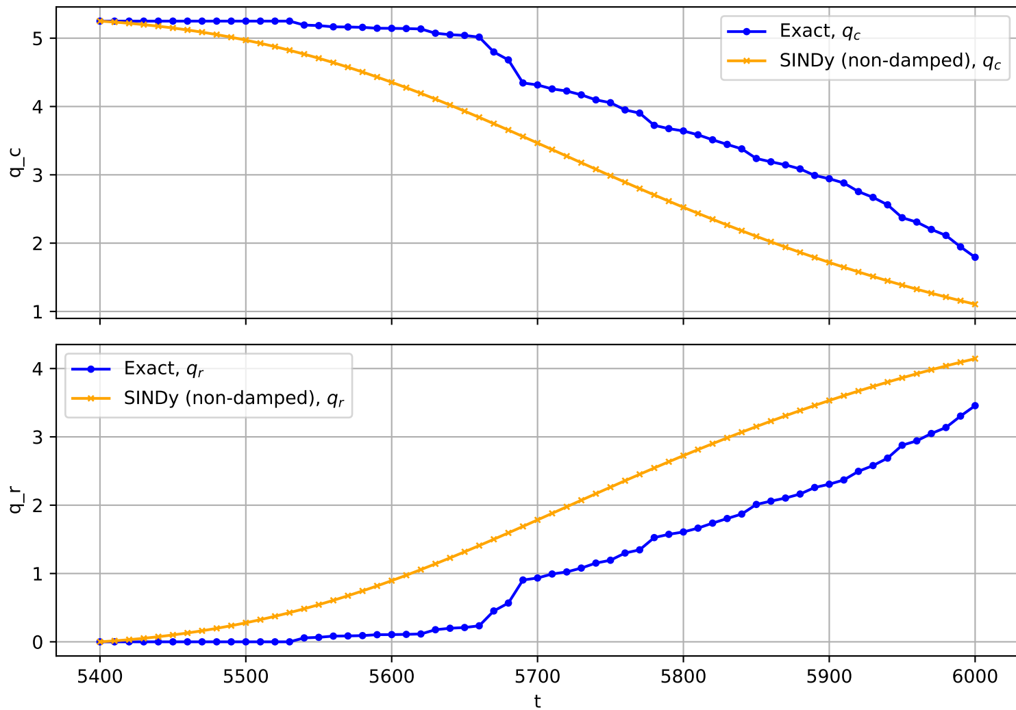
Trajectory No. 974
