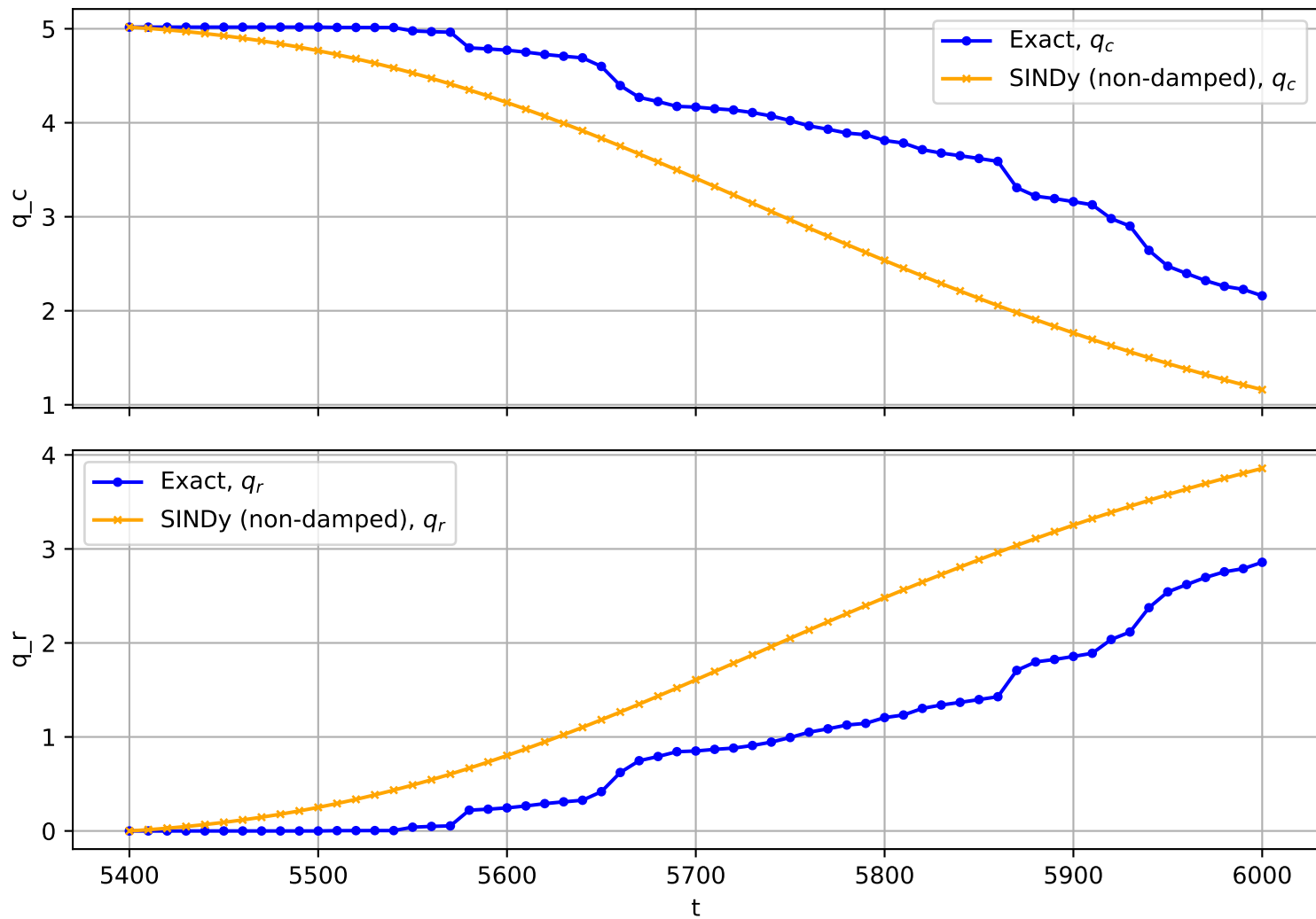
Trajectory No. 978
