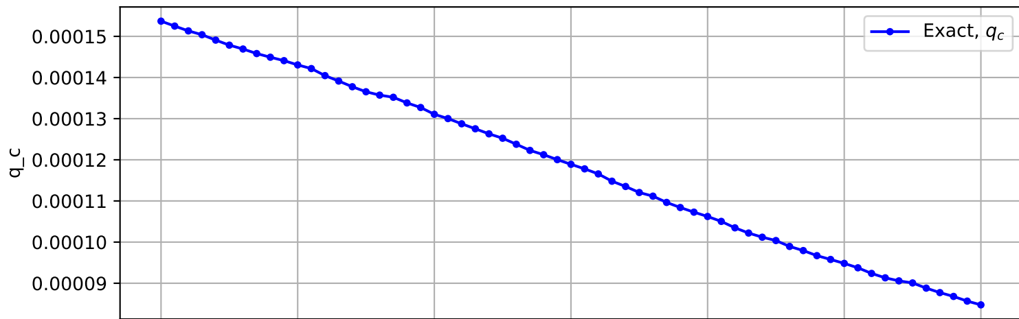
Trajectory No. 1048
